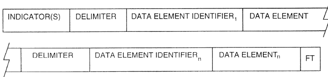
Figure 5 – Structure of a Variable Data Field
